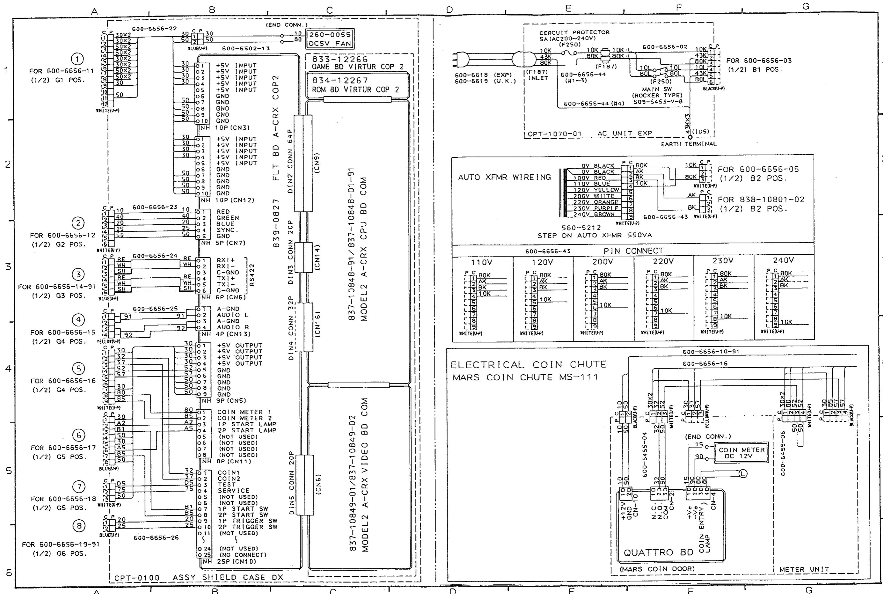
19. WIRING DIAGRAM (D-2/2)
