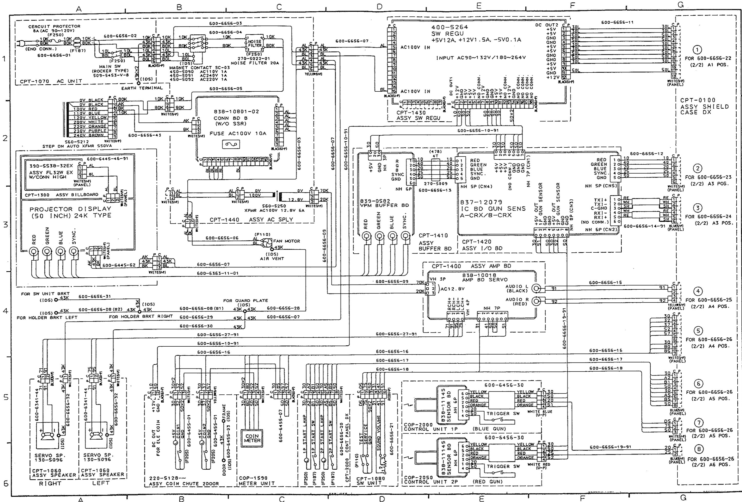
19. WIRING DIAGRAM (D-1/2)
