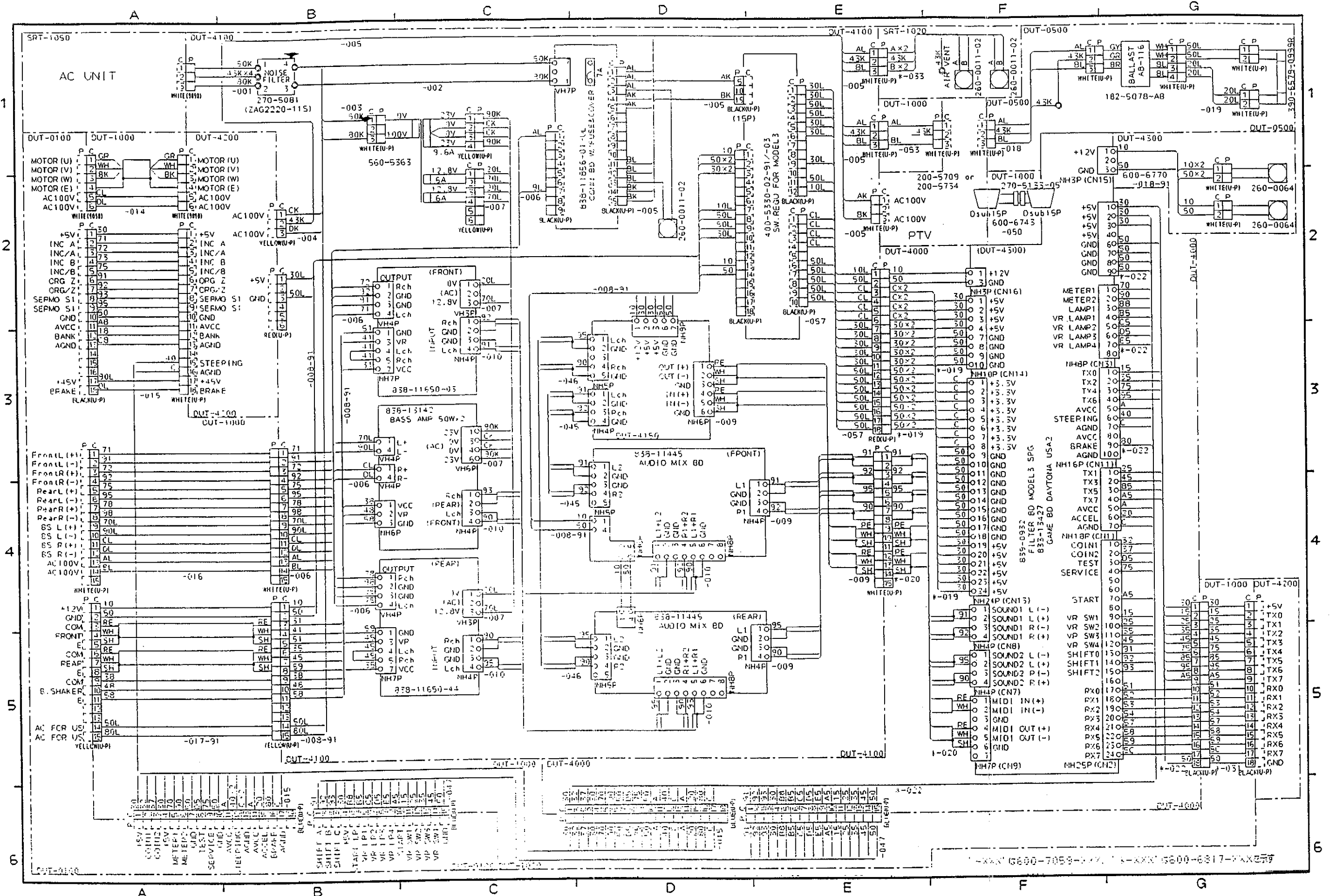
24. WIRING DIAGRAM (D-1/3)
