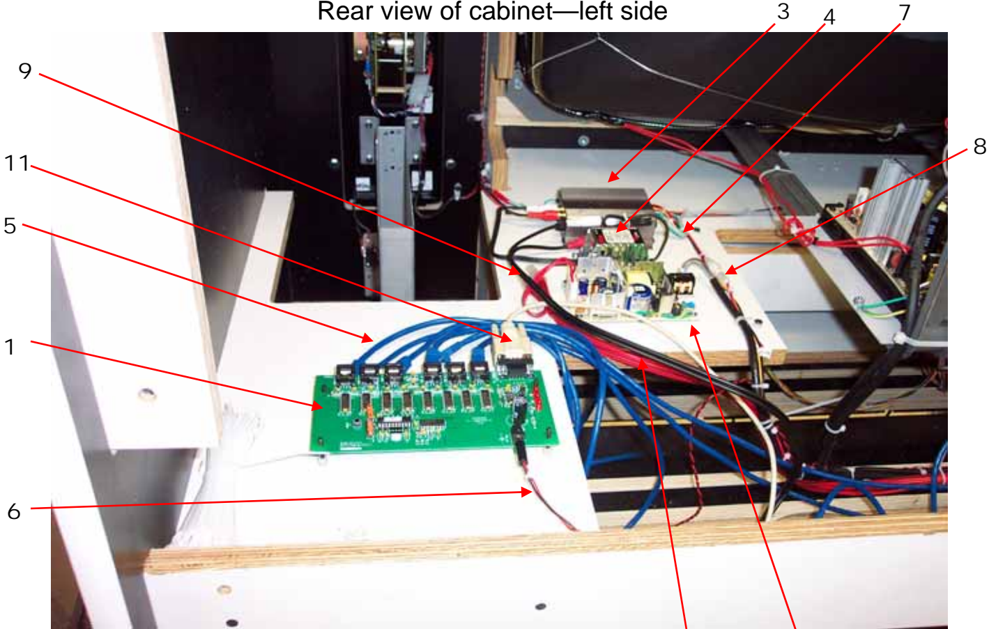
Rear view of cabinet—left side
