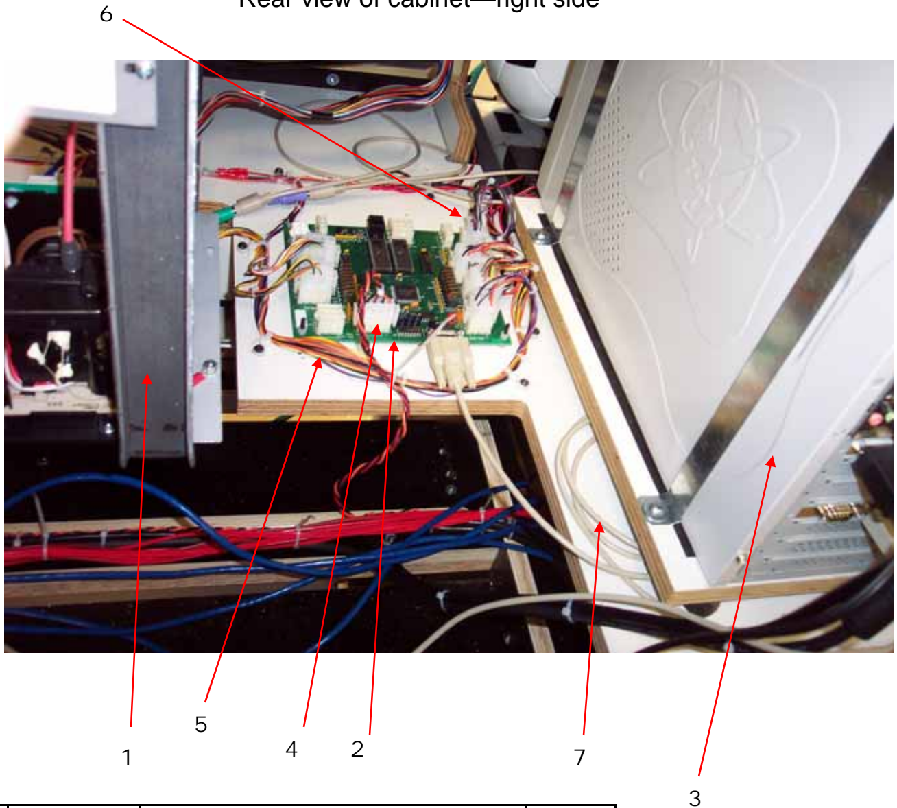
Rear view of cabinet—right side
