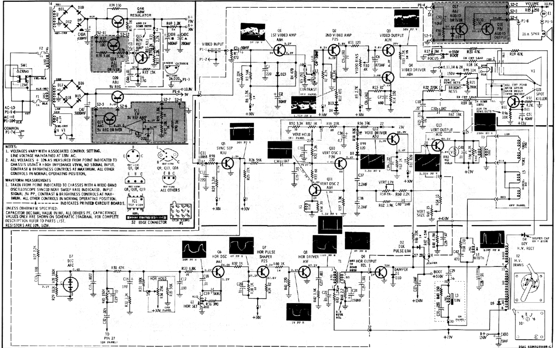
Schematic Diagram
