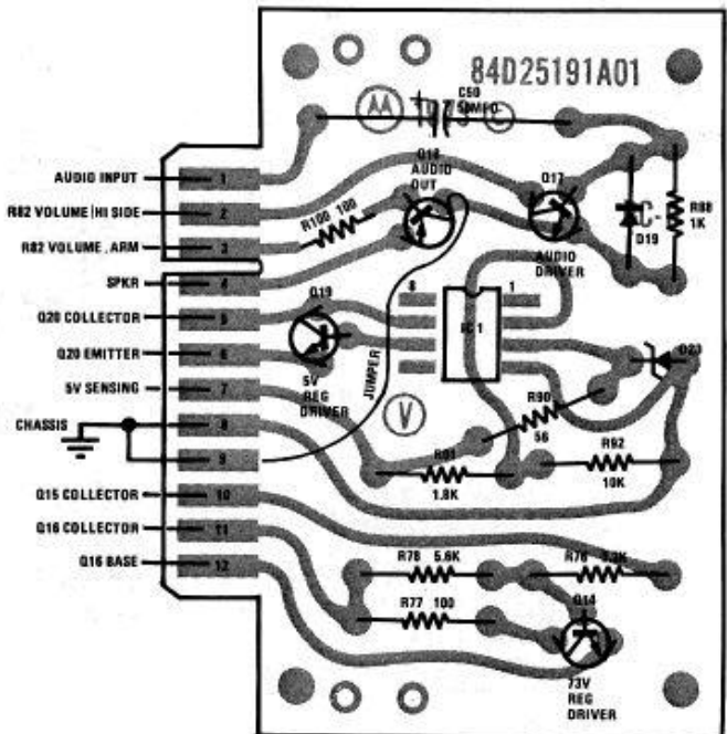
Circuit Side
