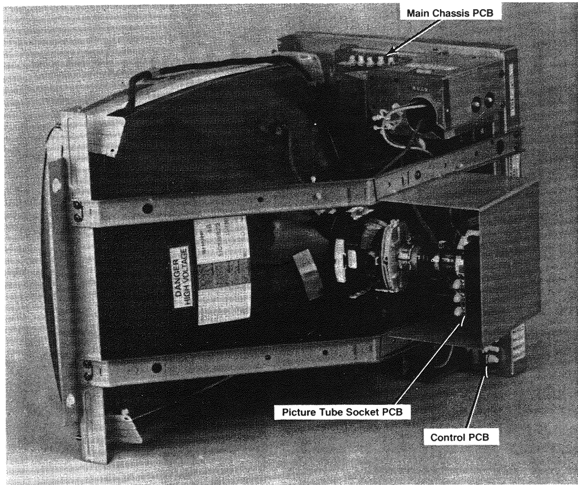
Figure 1 Overview of Sharp 19-Inch Color Raster Display
