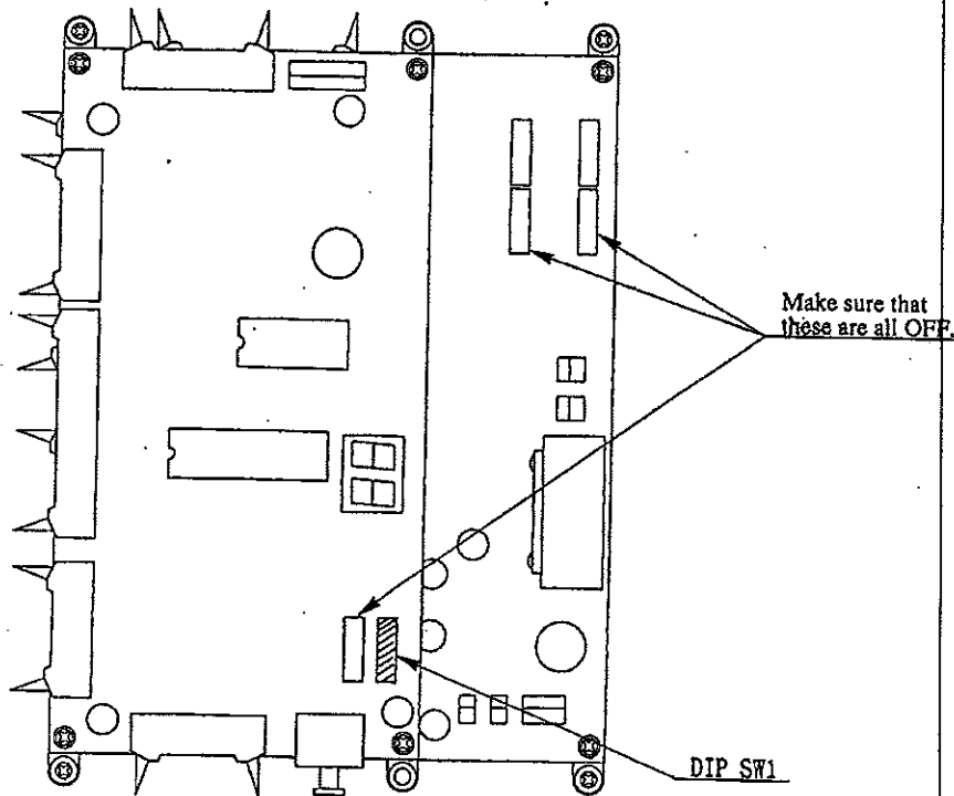
Fig. 11.3 CONTROL TOWER
