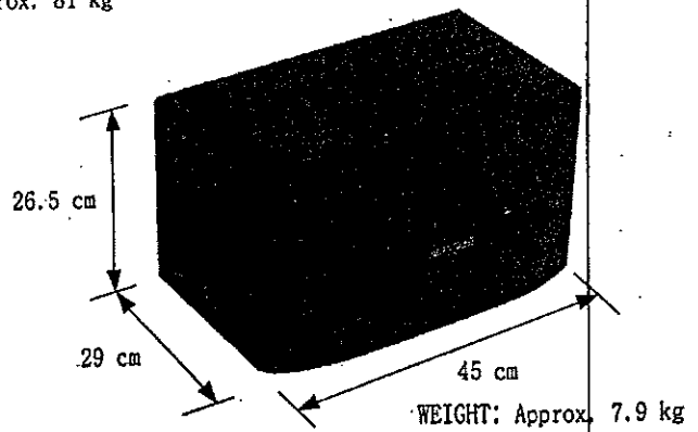
Fig. 5.7 SPEAKER[2]
