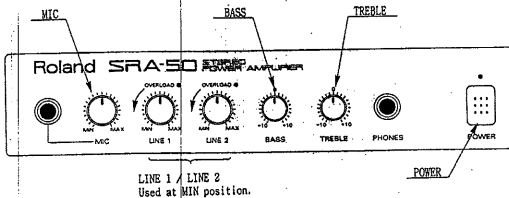
Fig. 11.2 POWER AMPLIFIER
