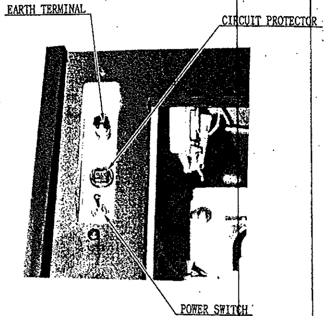
Fig. 17.1 CIRCUIT PROTECTOR
