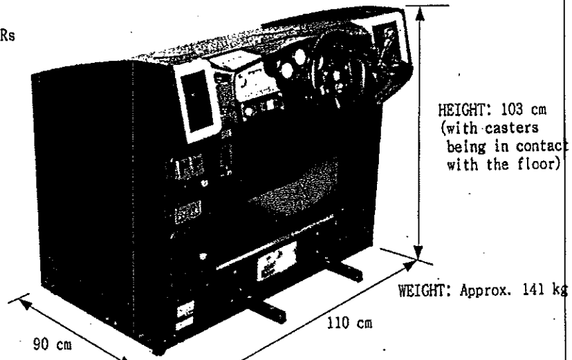
Fig. 5.4 FRONT CABI[8(4)]
