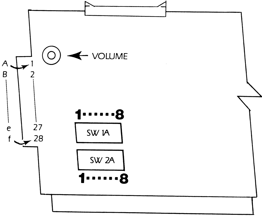
PCB Layout
