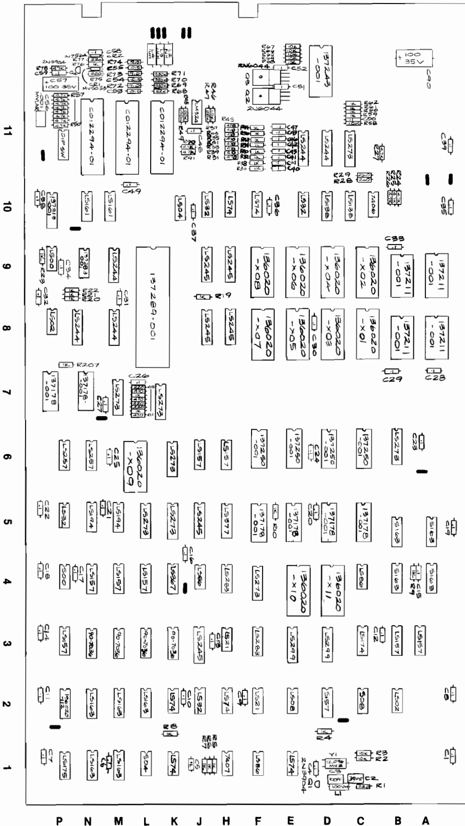
Figure 3-14 Food Fight Game PCB Assembly A039445-21 B
