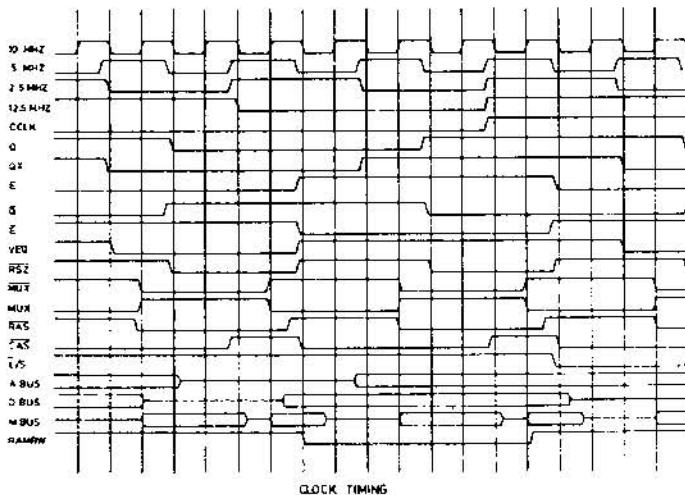
FIGURE 3-1 CLOCK TIMING
