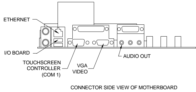
FIGURE 29 - ECS MOTHERBOARD DRAWING
