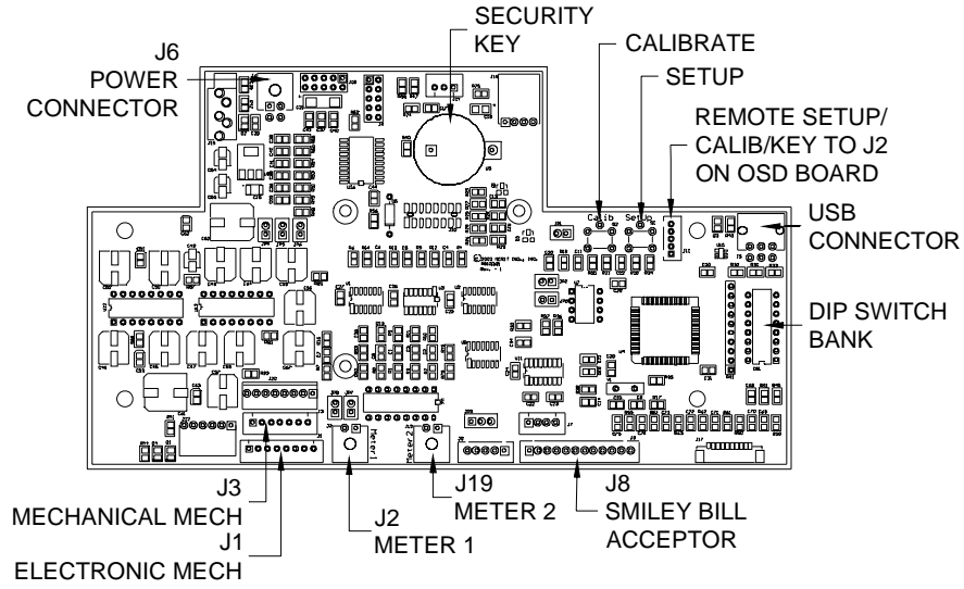
FIGURE 29 - I/O BOARD DRAWING
