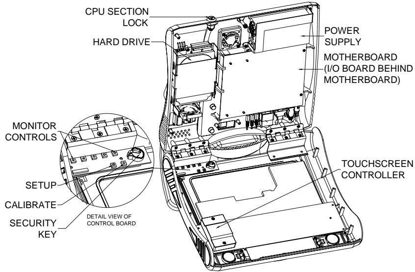
FIGURE 24 - THE EVO WITH CPU SECTION OPEN
