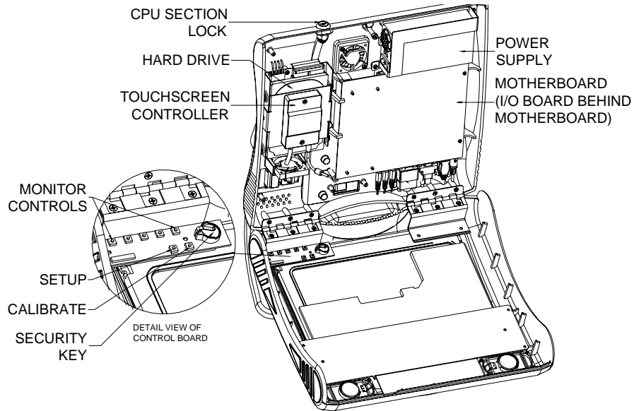
FIGURE 1 - EVO WALLETE WITH CPU SECTION OPEN
