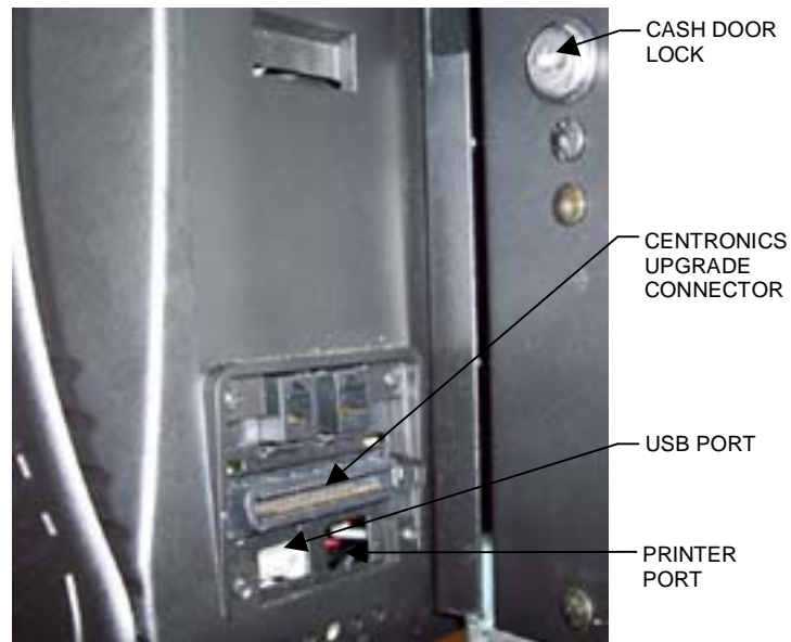
FIGURE 2 - REAR VIEW OF EVO WALLETE - CPU SECTION SLID TO THE LEFT (COVER PLATE OVER COMMUNICATIONS MODULE SECURED BY 5/64" ALLEN SCREW)
