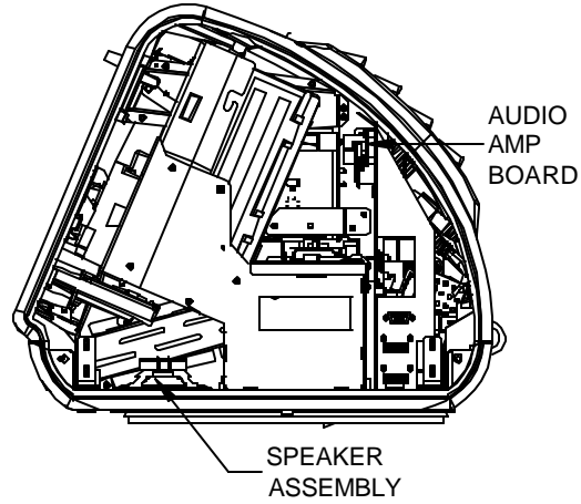
FIGURE 3 - LOCATION OF EXISTING SPEAKER ASSEMBLY/AUDIO AMP BOARD
