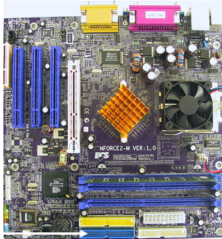
FIGURE 1 - ION ECS MOTHERBOARD
