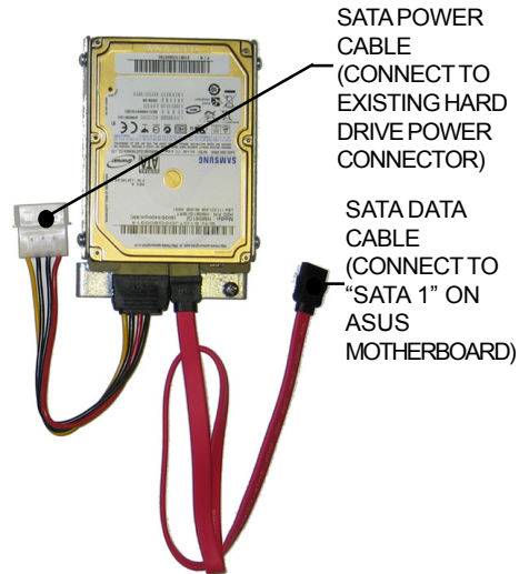
FIGURE 4 - NEW SATA HARD DRIVE ASSEMBLY FOR GAMES WITH ASUS MOTHERBOARDS, AND FOR WIDESCREEN AURORAS AND RX GAMES
