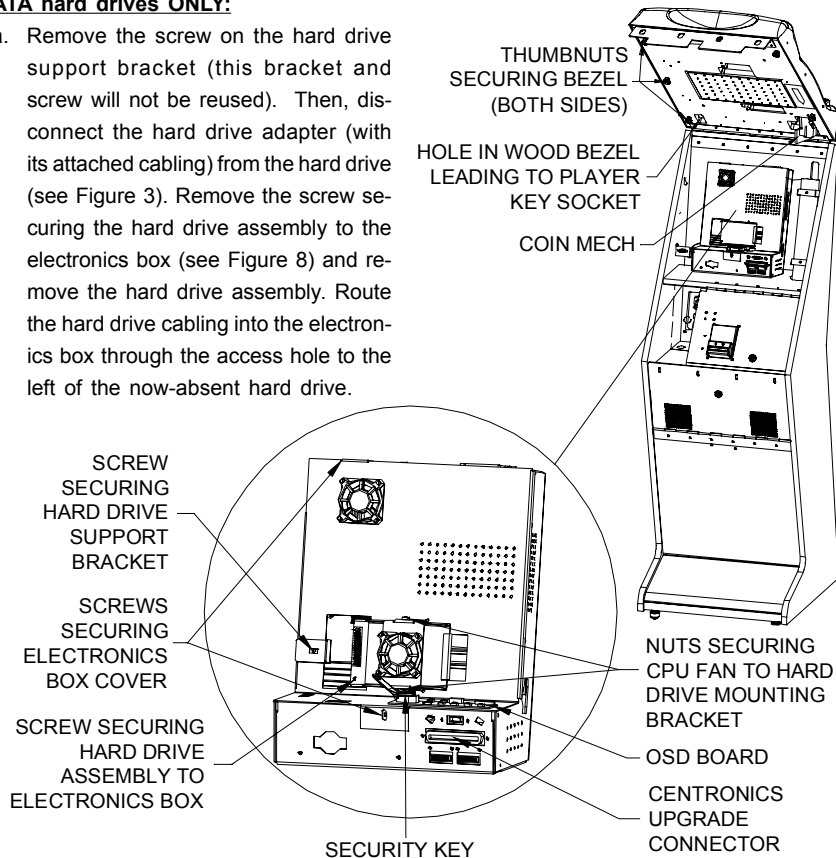
FIGURE 8 - FUSION GAME WITH DETAIL VIEW OF ELECTRONICS BOX
