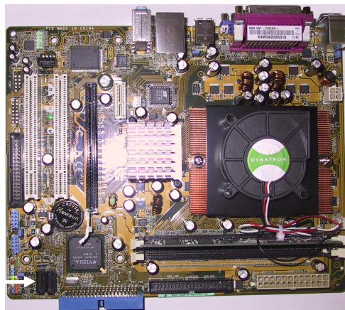
FIGURE 2 - ION ASUS MOTHERBOARD
