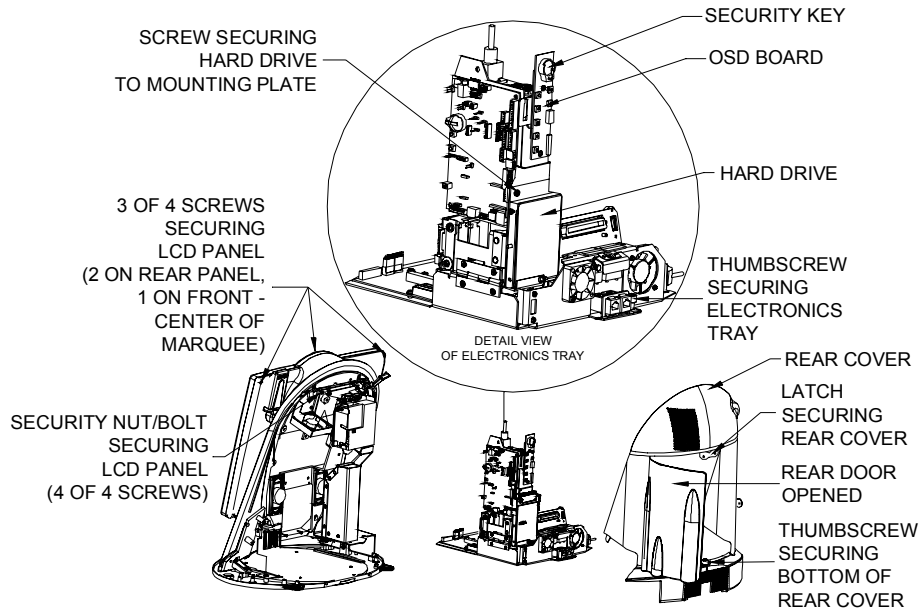
FIGURE 12 - REAR VIEW OF AURORA WIDESCREEN GAME
