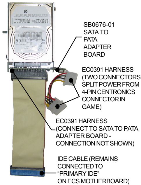
FIGURE 5 - NEW SATA HARD DRIVE ASSEMBLY FOR EVO, EDGE, & WALLETT/ENTERTAINER GAMES WITH ECS MOTHERBOARDS
