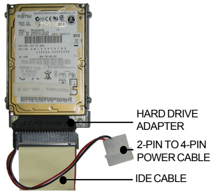
FIGURE 3 - OLD PATA HARD DRIVE ASSEMBLY
