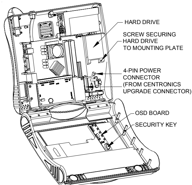
FIGURE 7 - EVO, EVO WALLETTTE / ENTERTAINER, AND ELITE EDGE WITH CPU SECTION OPEN
