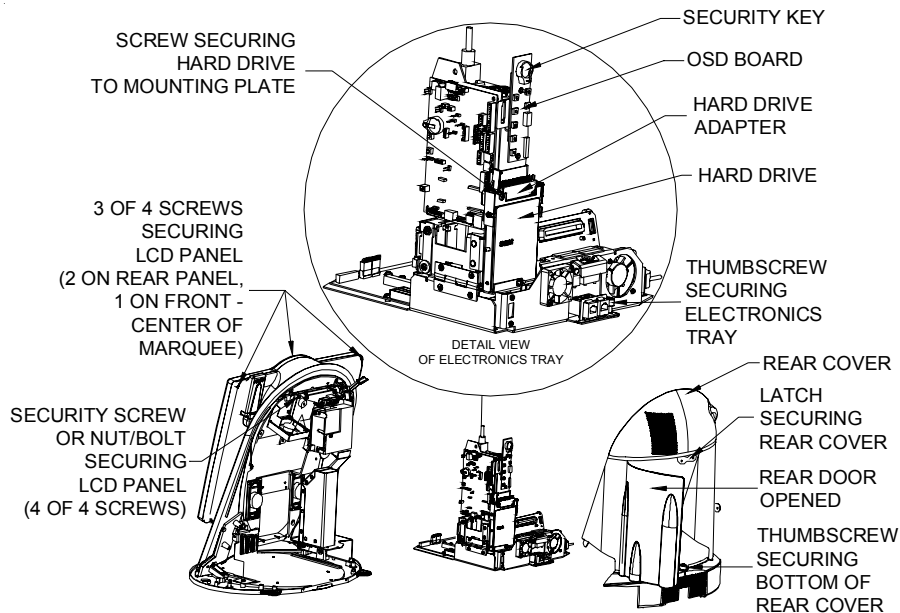
FIGURE 11 - REAR VIEW OF AURORA GAME
