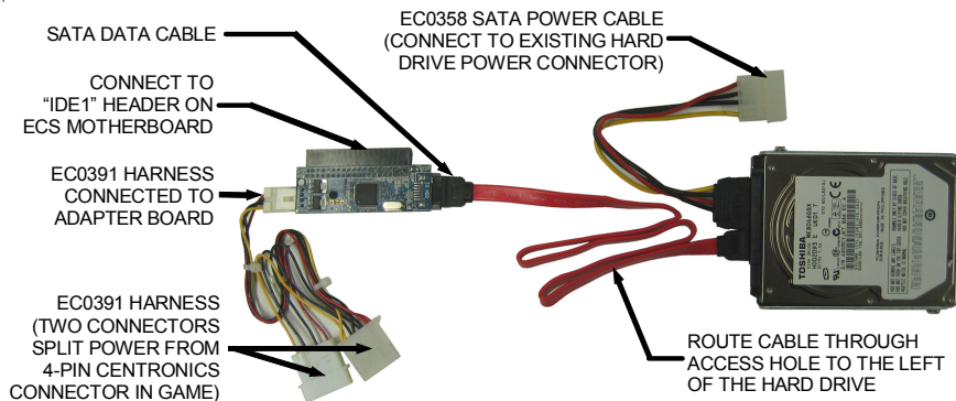
FIGURE 9 - SATA TO PATA ADAPTER BOARD AND CABLING (ECS MOTHERBOARDS ONLY)
