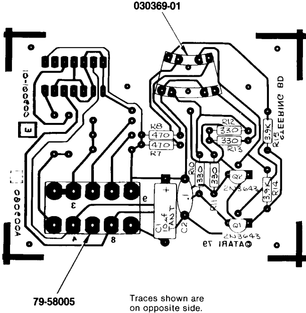
Detail of Steering PCB Assembly, A009060-02, Rev. C:
