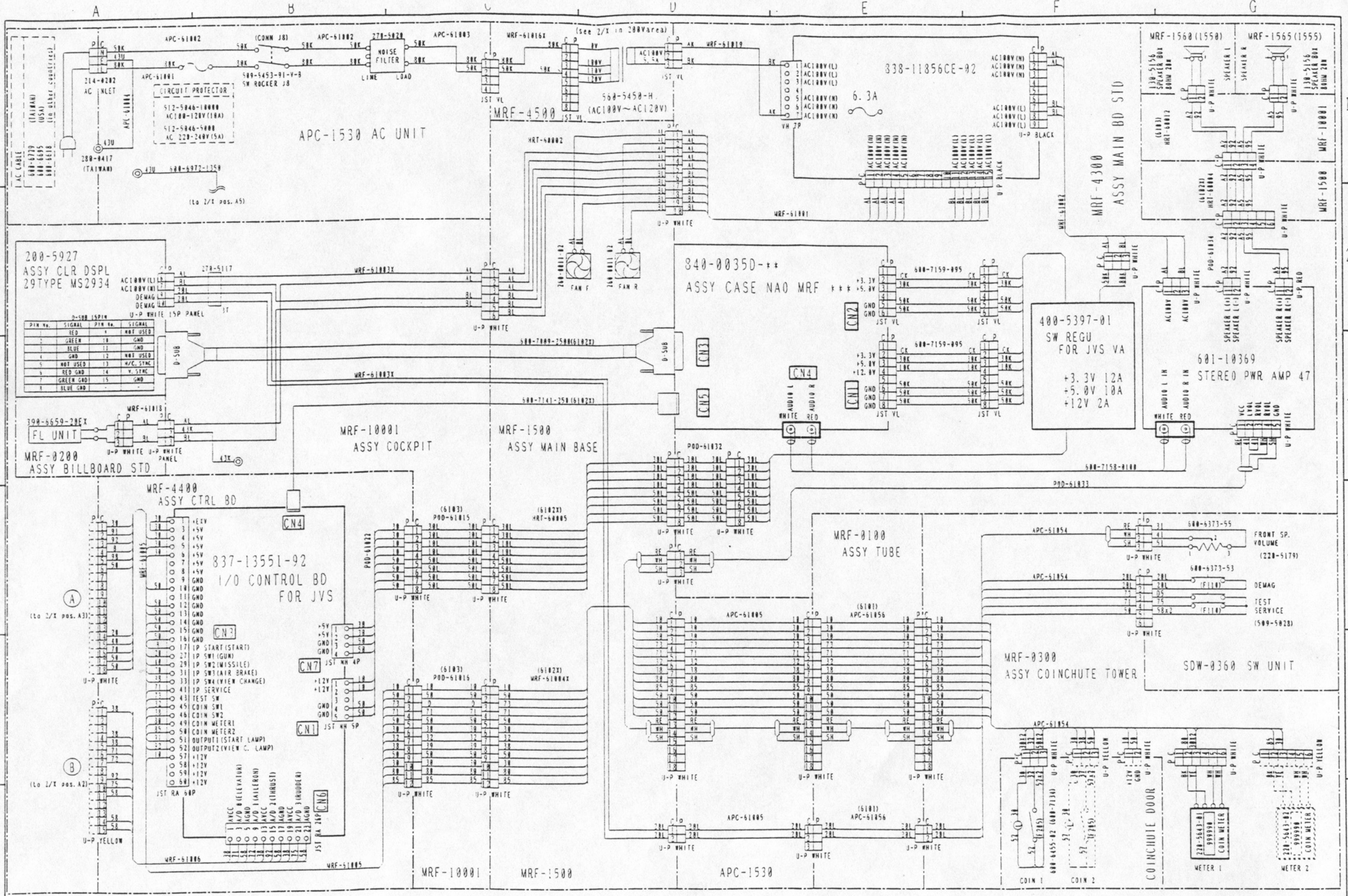
21. WIRING DIAGRAM (D-1/2)
