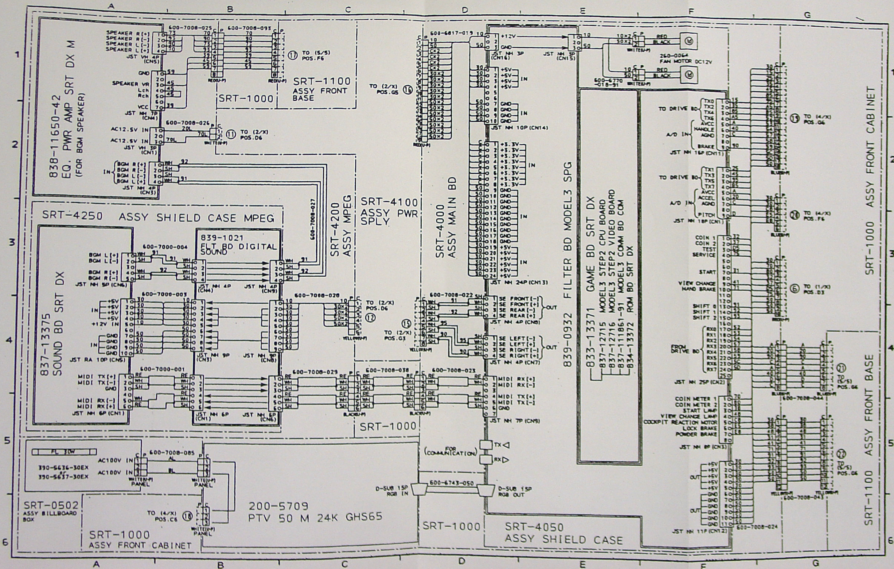
WIRING DIAGRAM (D-3/5)
