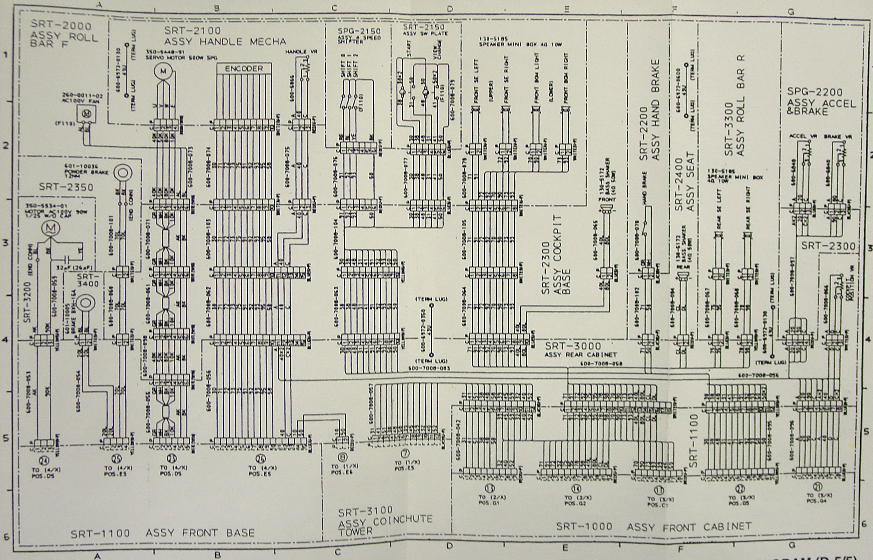
WIRING DIAGRAM (D-5/5)
