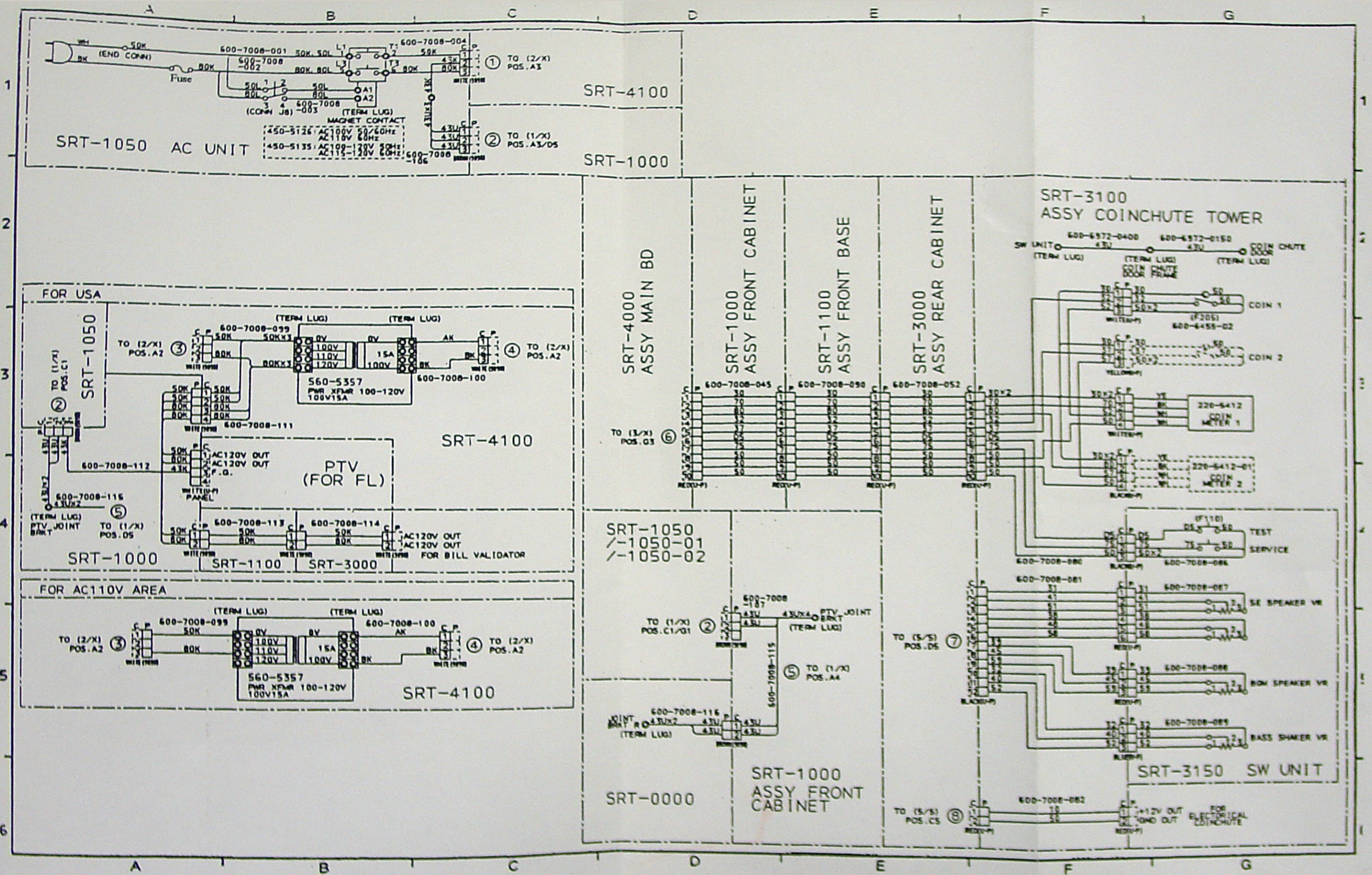
WIRING DIAGRAM (D-1/5)
