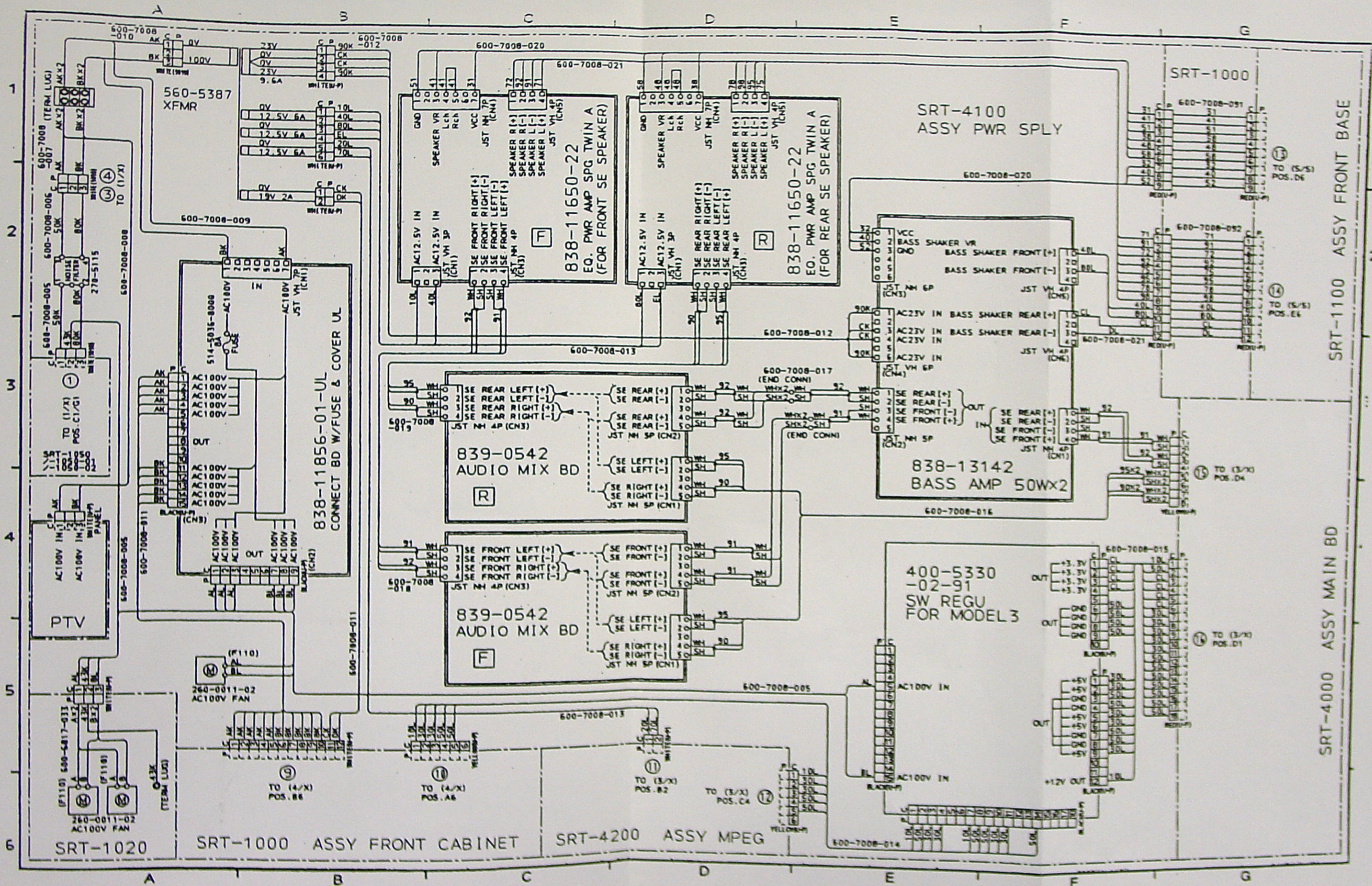
WIRING DIAGRAM (D-2/5)
