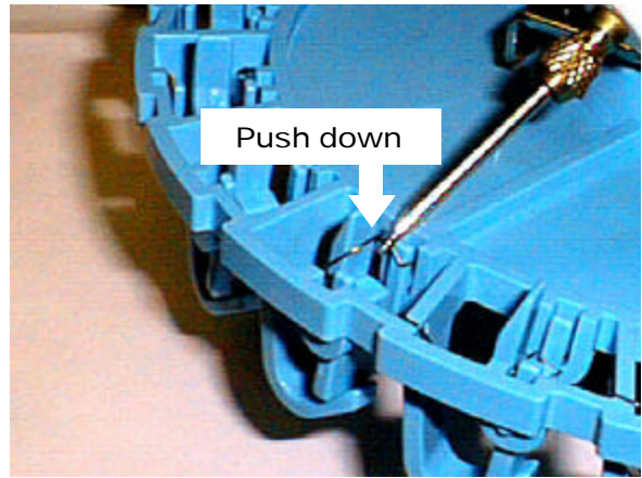
6) After Hooked, push down the Spring over Latch.
