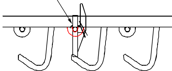
Back Side View of Latch & Spring
