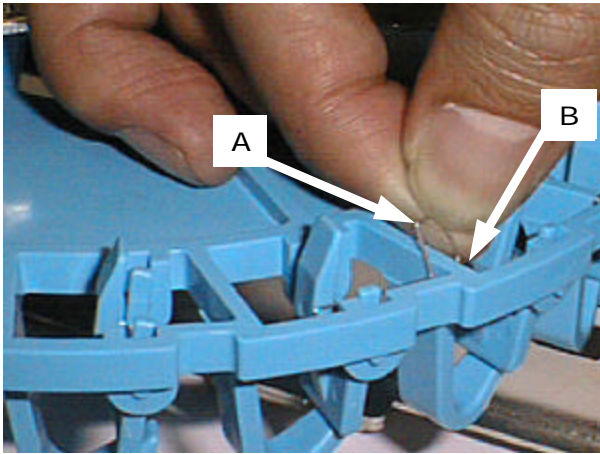
3) Hook part A of SPRING over part B of Hanger as far forward as possible.
