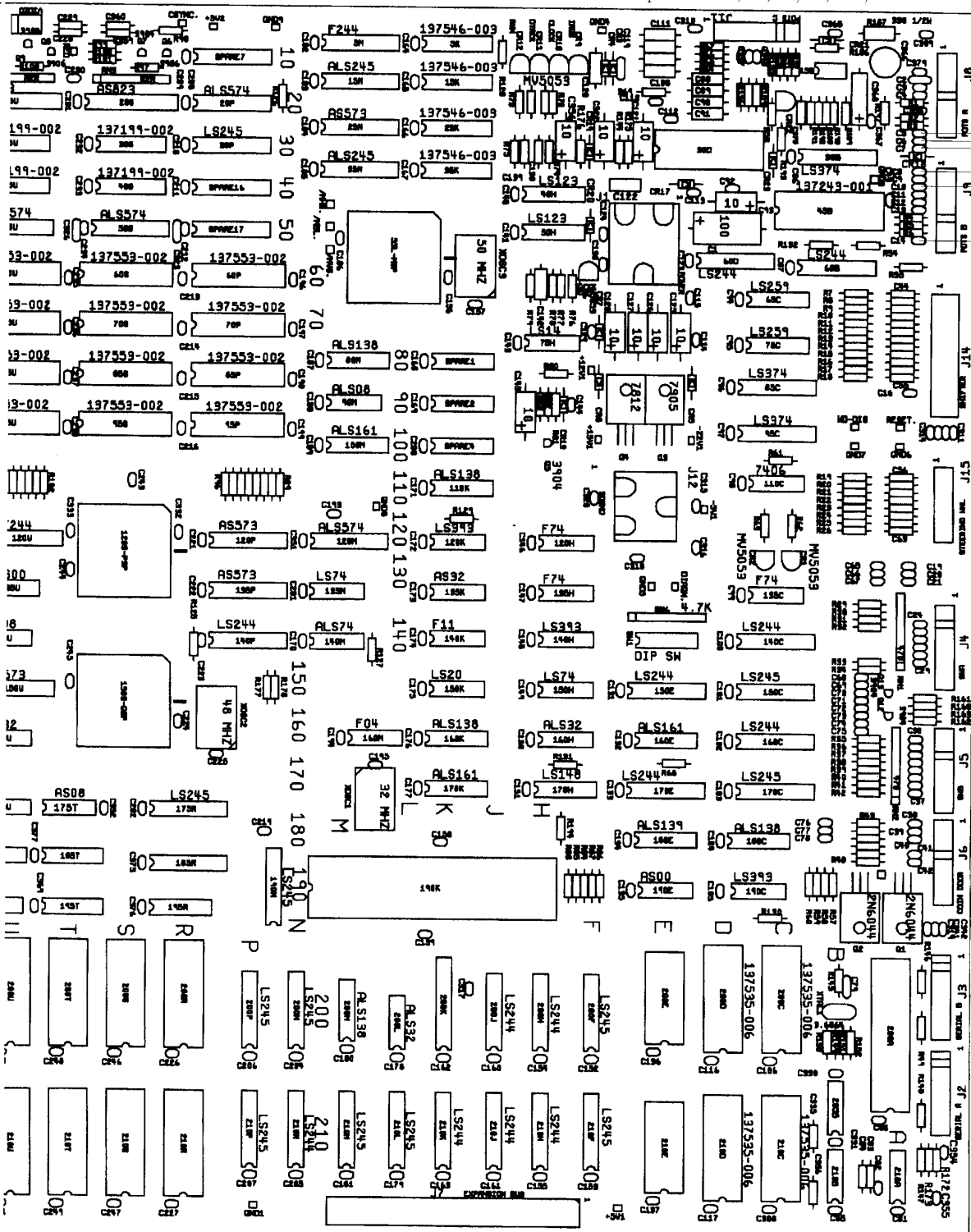
Figure 4-8 Multisync PCB Assembly, Continued A044998-03 B
