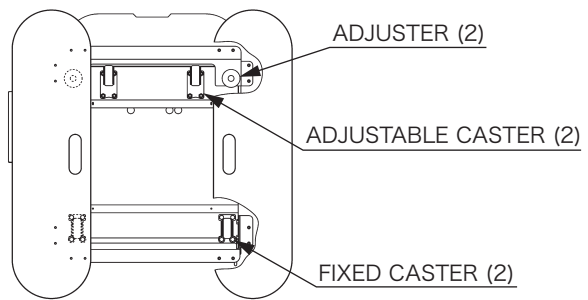
FIG. 6.1 a Bottom View
