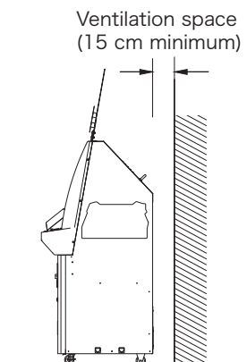
FIG. 6.1c Ensuring Ventilation Space
