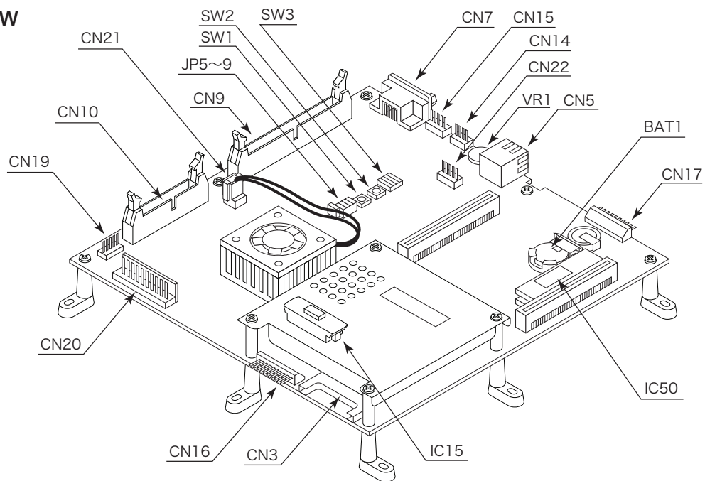
FIG. 10.1 SystemSP Board External View
