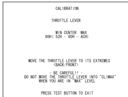
[THROTTLE LEVER (STEP2-2) Screen] (test_calibrate_throttle_3.jpg)
