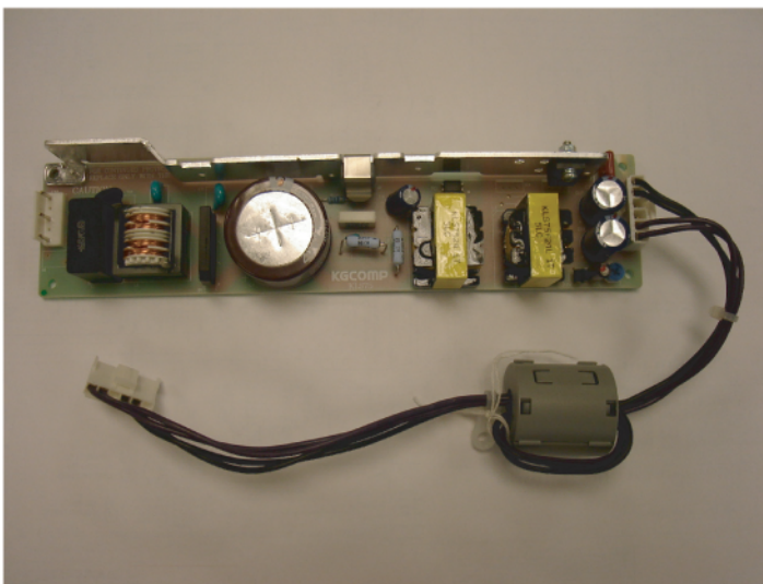
998-0248 POWER SUPPLY(KGCMP)
