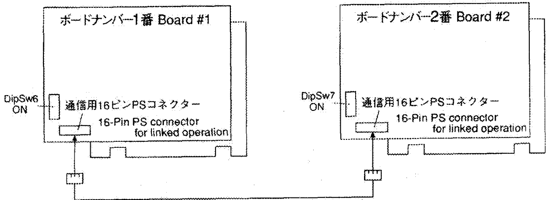
Connection for Two Boards Linked Operation
